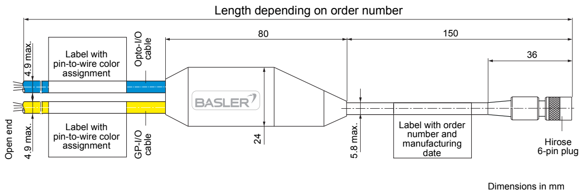
Fig. 1: Cable Overview
