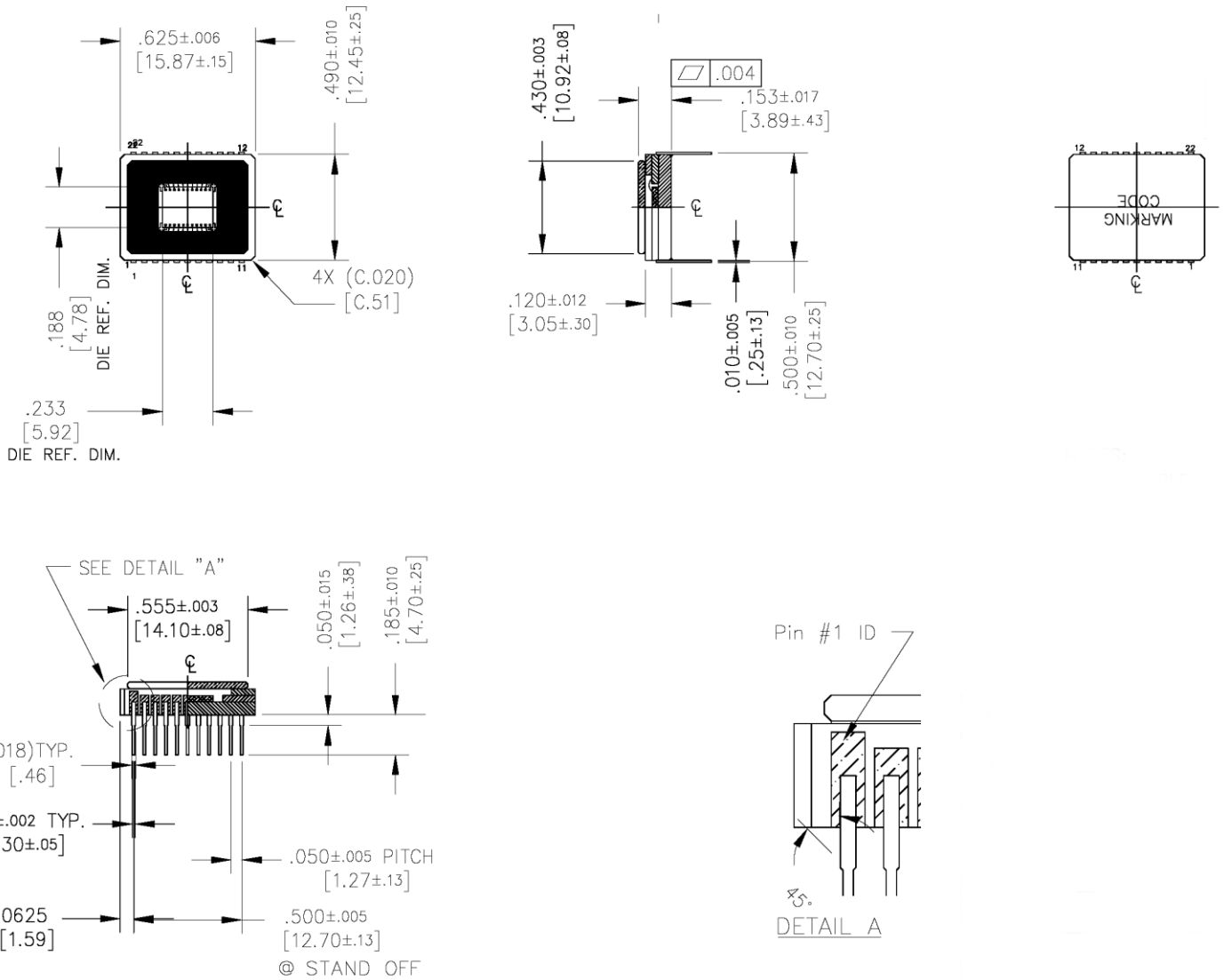
Figure 21: Completed Assembly
