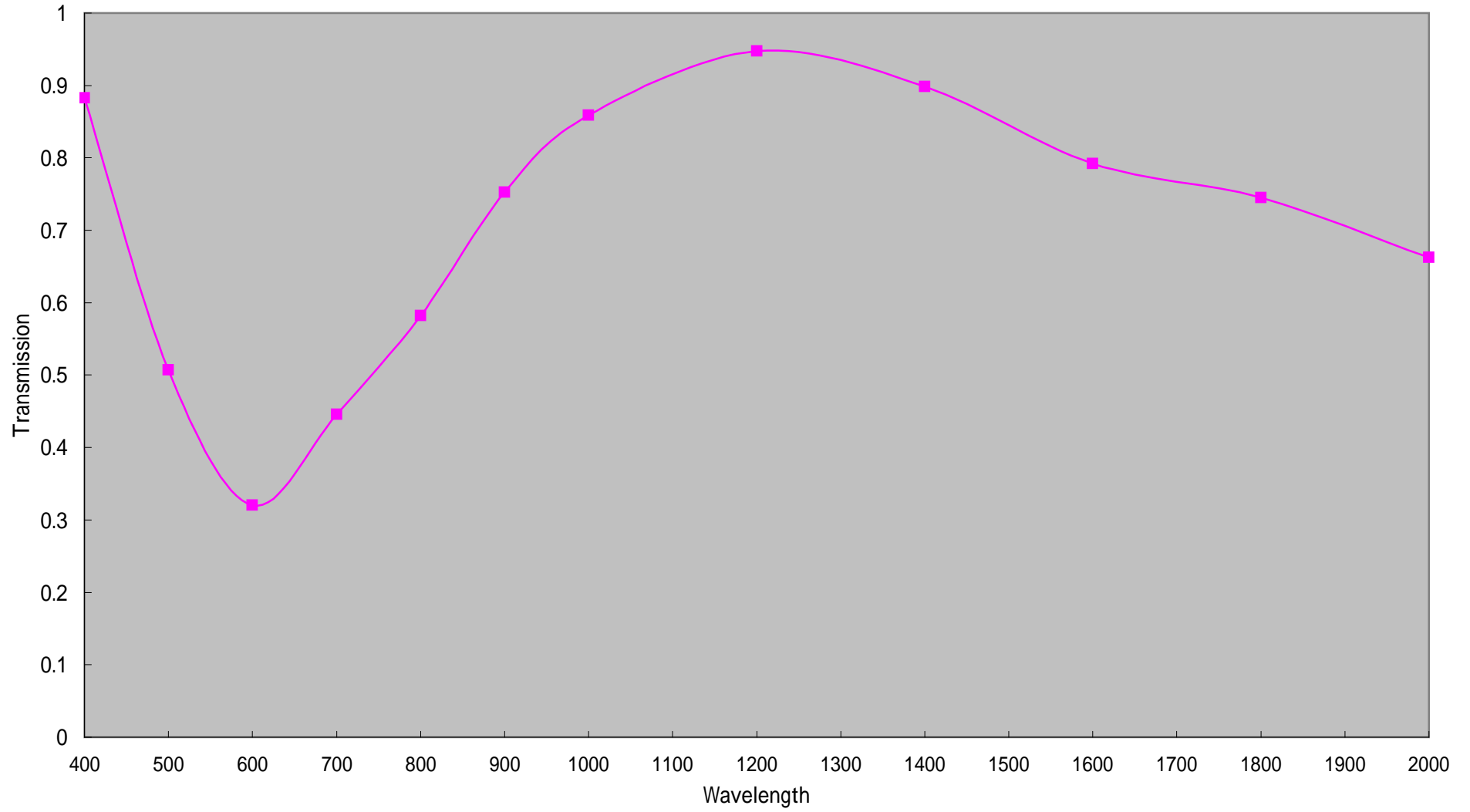
LM25HC-SW Transmission
